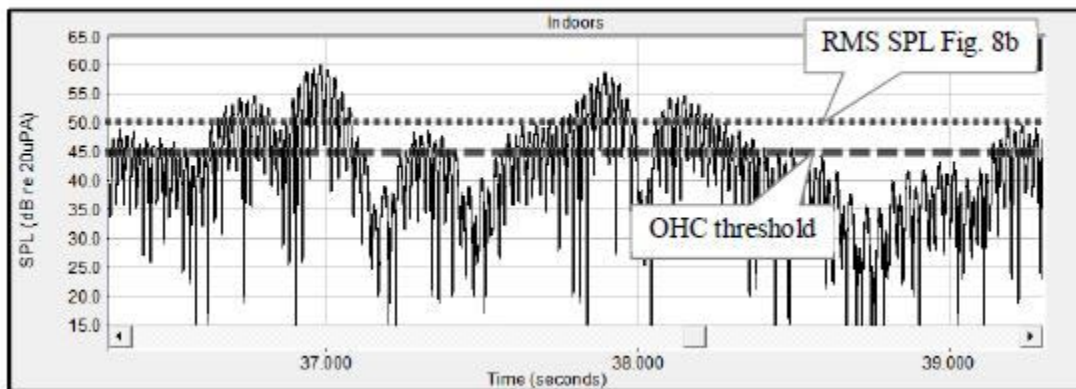
Figure 9 – 22.9 Hz tone and its OHC threshold
